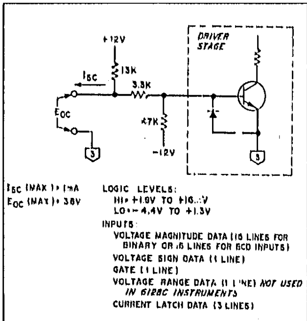
Figure C-2, Receiver Circuit
