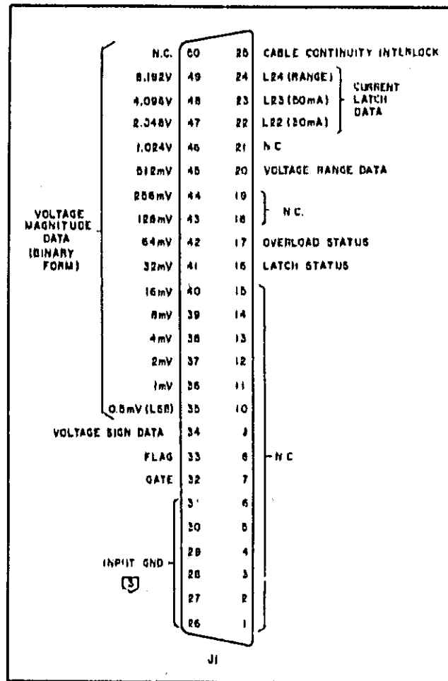
Figure A-1. Input/Output Data Connector
