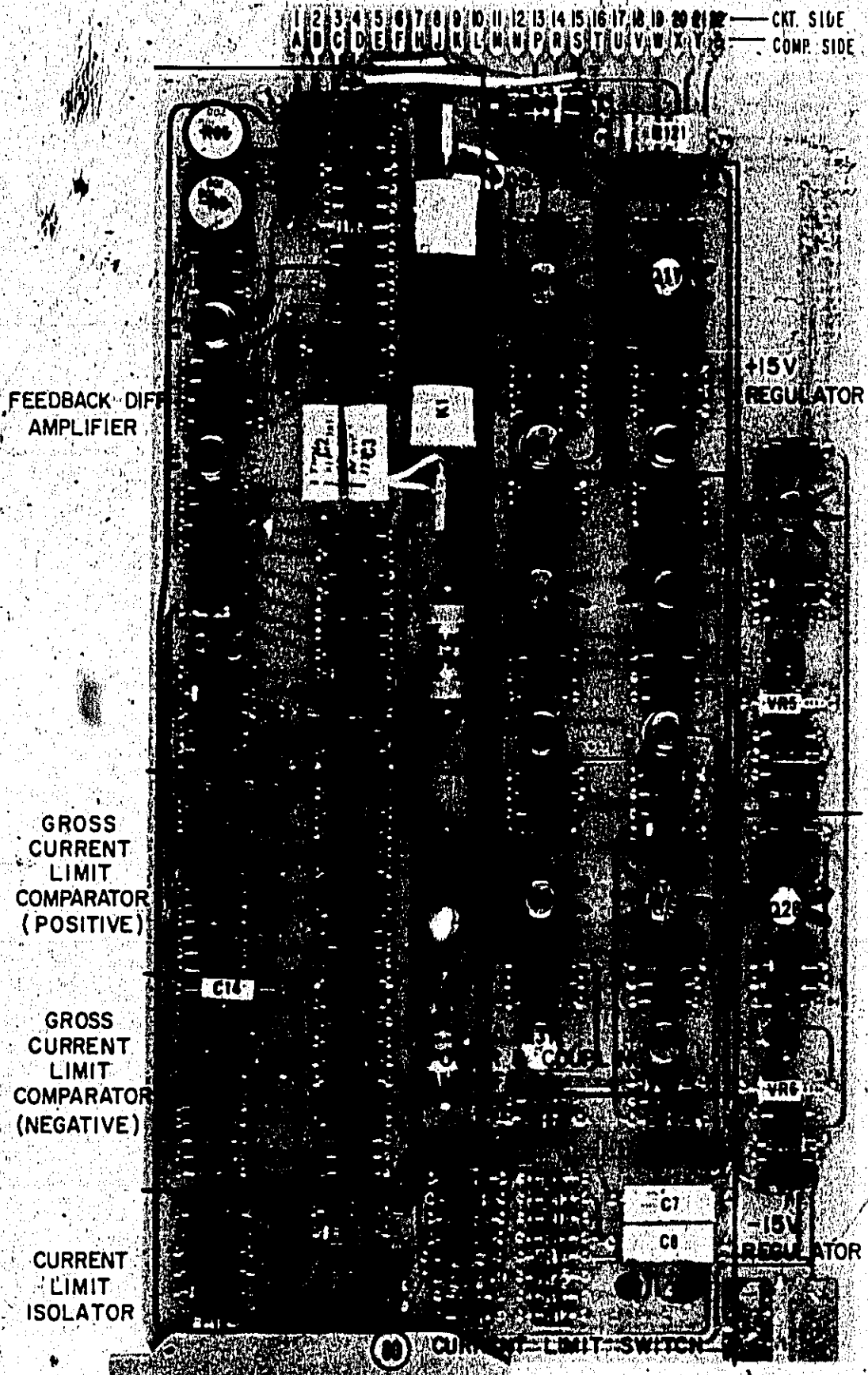
A7 Amplifier Board, Component Location
