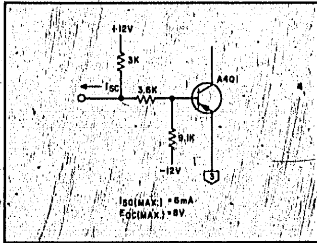
Figure C-3. Cable Continuity Interlock Receiver Circuit.
