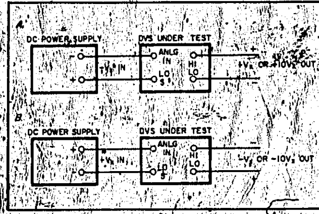
Figure 5-7. DVS Analog Input Connections
