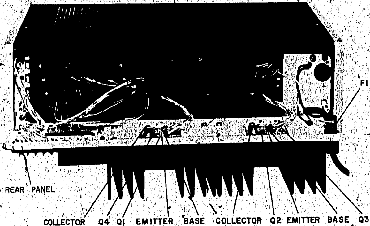
Rear View, Component Location.
