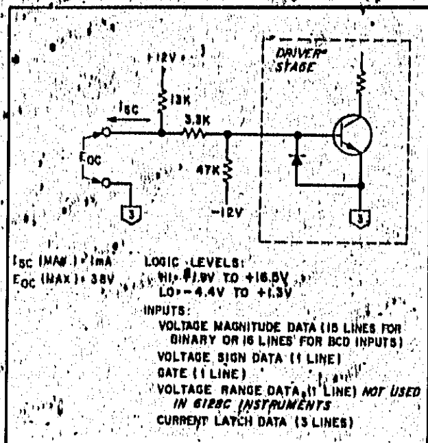
Figure C-2. Receiver Circuit
