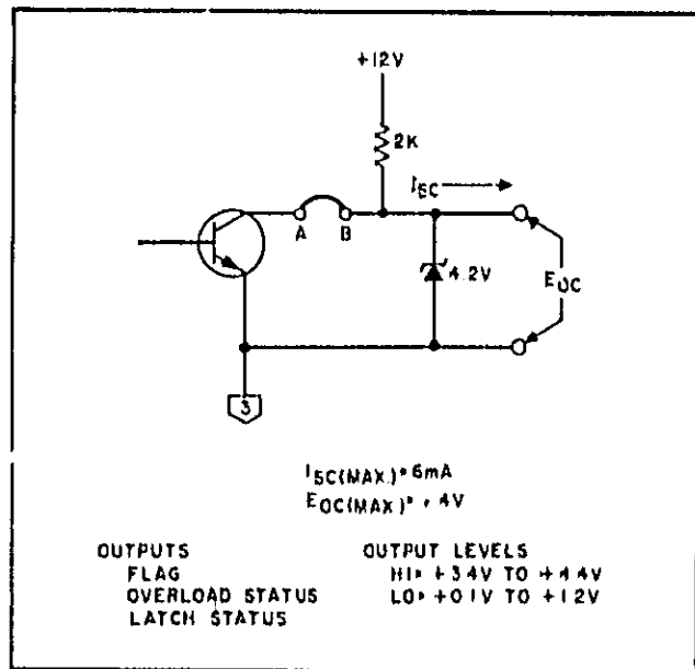
Figure C-4, Driver Circuit
