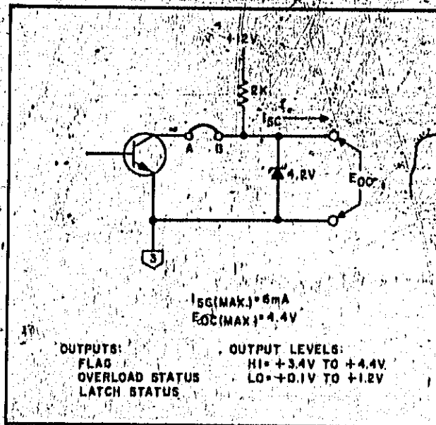
Figure C-4. Driver Circuit.
